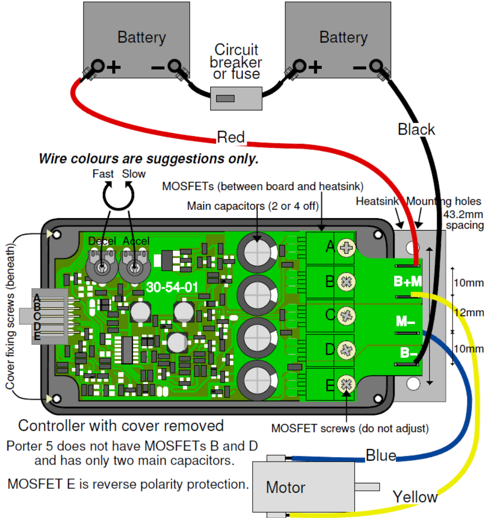
Figure 1: Porter Wiring
